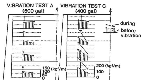
Fig. 6 Maximum reinforcement tensile force during vibration
