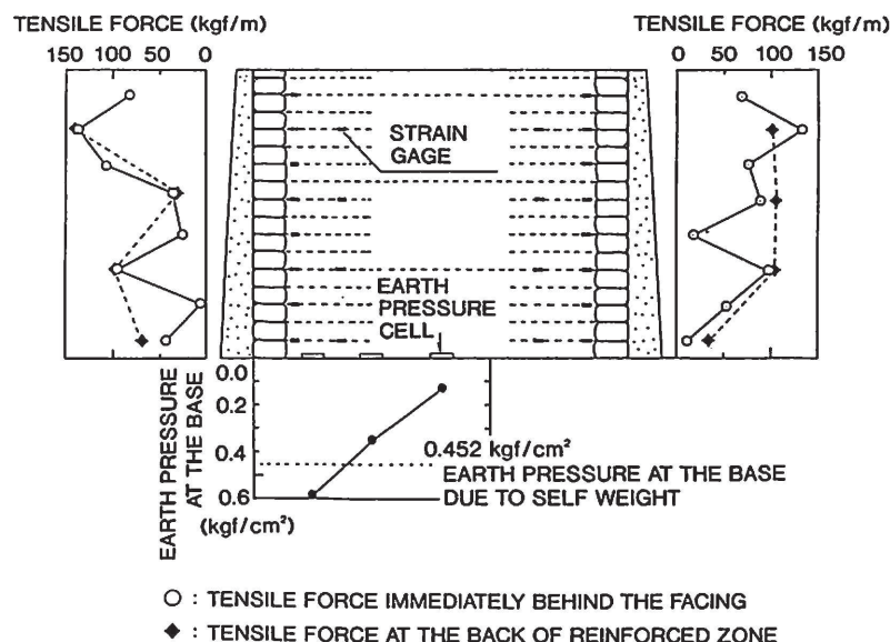
Fig. 2 Earth pressure and reinforcement tensile force after construction
