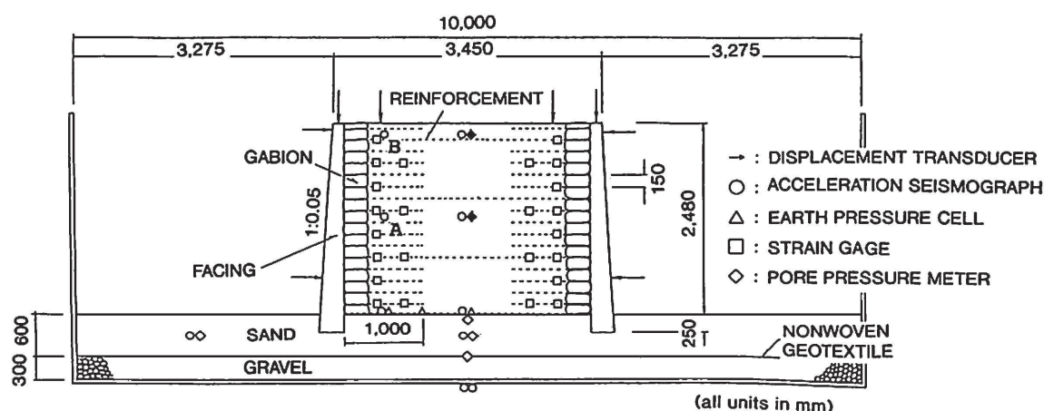
Fig. 1 Configuration of large scale model and instrumentation
