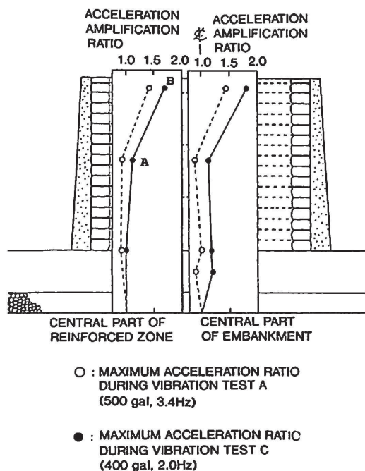
Fig. 4 Acceleration amplification ratio in the embankment
