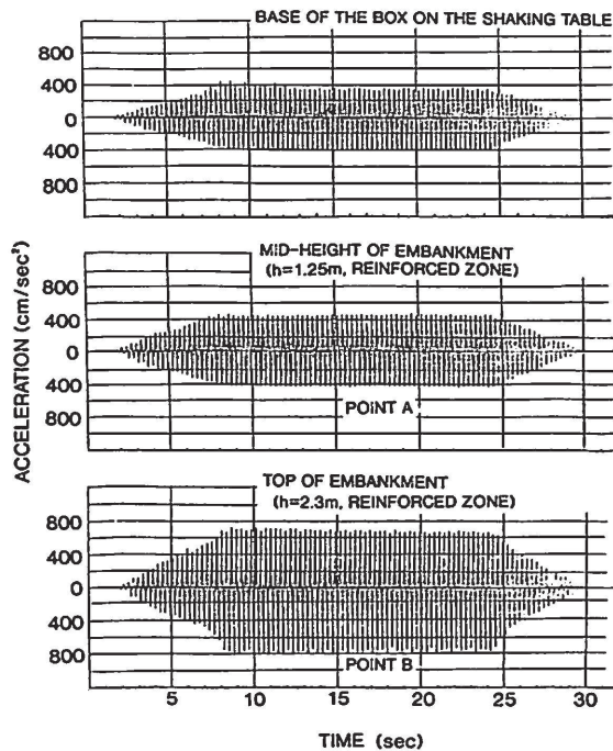
Fig. 3 Measured acceleration versus time (Vibration Test A)
