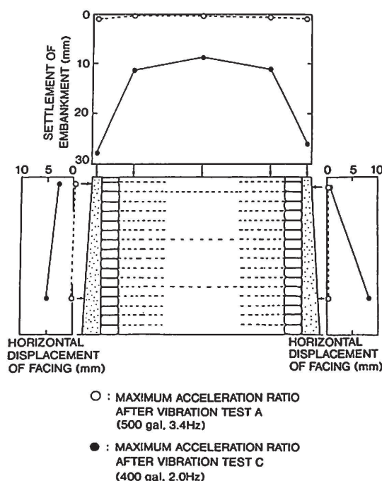
Fig. 5 Maximum deformation of the embankment after vibration
